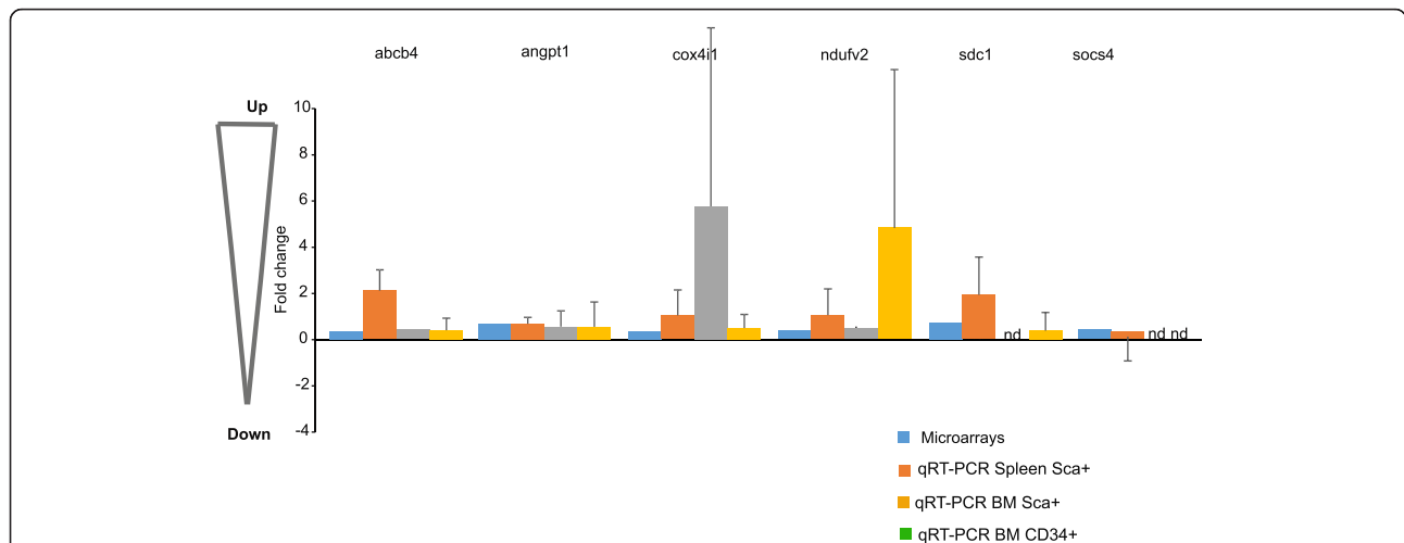
Fig. 4 qRT-PCR validation of the GEP microarray data (blue) in Sca1+ cells purified from BM or spleen of another set of HR-MDS mice (two different hues of orange), and CD34+ cells purified from MDS patients (green) compared to FBV/N or CD34 BM cells, respectively. Data expressed as fold change of expression of several genes of three pathways shown (angpt1 (signal transduction); cox4i1 and ndufv2 (oxidative metabolism); sdc1 (DNA processing)). qRT-PCR fold changes shown here are represented as the average of three experiments
